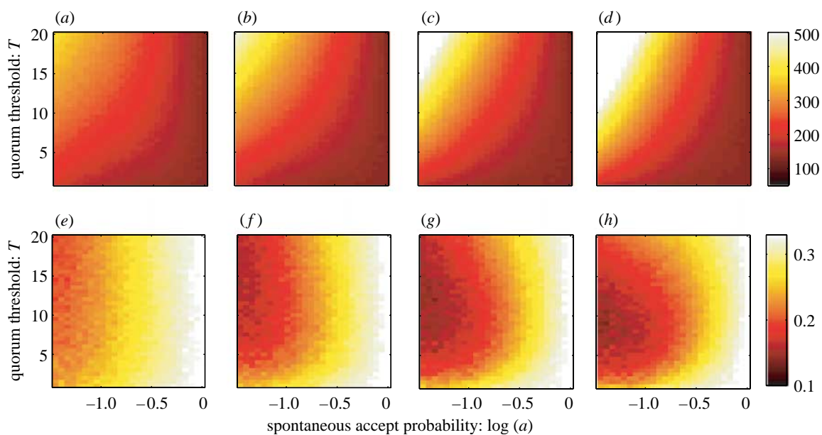
Figure 5. Speed and accuracy of decision making for the simple quorum response model. Predicted effects of the parameters a , T and k on ( a – d ) the time until all individuals have made a decision and ( e – h ) the accuracy of that decision. In each image, a and T are varied for different threshold steepness, k . The plots show mean duration (time steps of the model) and accuracy (proportion of individuals choosing the less attractive option Y ) over 1000 simulations for each parameter combination. ( a ) k=1 ; ( b ) k=2 ; ( c ) k=4 ; ( d ) k=9 ; ( e ) k=1 ; ( f ) k=2 ; ( g ) k=4 ; ( h ) k=9 .
